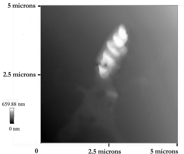
FIG. 11: AFM of double-helix rods: Taken 90 minutes after droplet laid out to dry on graphite. A trail of amorphous water structure can be observed at the lower end of the rod. It may be water expelled from the double helix, or it may be surrounding water restructured.
